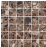
Corniola
