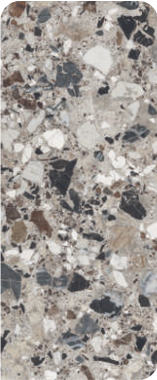
Diorite
